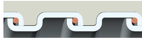
Square-Locked Design with integral bonding wire 3/8" through 1-1/4"
