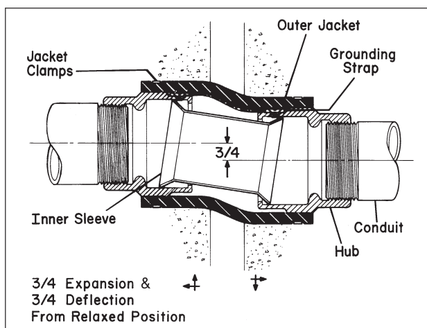
3. Parallel misalignment.
