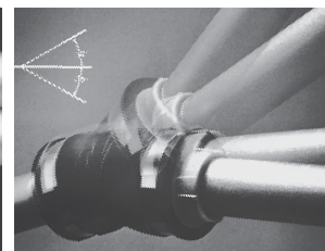
2. Angular misalignment.
