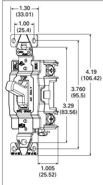
Figure 2. AH1220 Series
