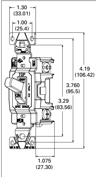
Figure 1. AH1200 Series
