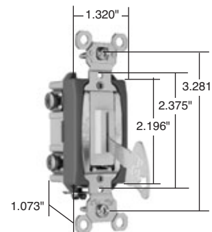
Dimensions for 15 & 20 Amp Locking
