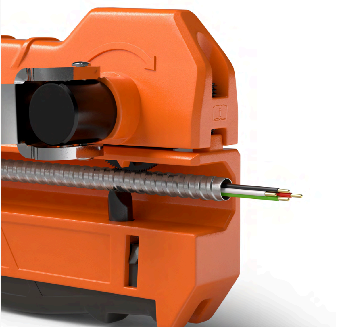
Quickly Cuts Through MC • BX • AC • MCAP • Greenfield
