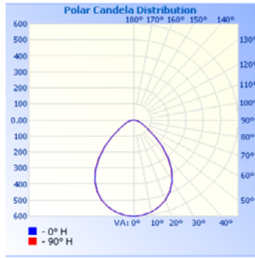
RT4S1000UNHD9SC3WH (2700K)
