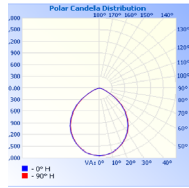
RT8S3500UNHD9SC3WH (2700K)
