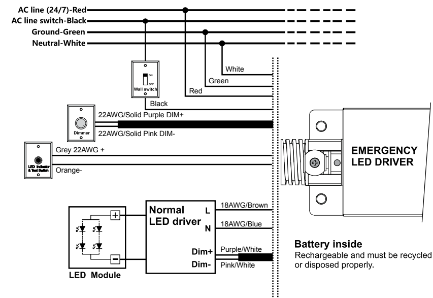
Wiring diagram
