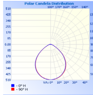
RT6S900UNVD9SC3WH (5000K)
