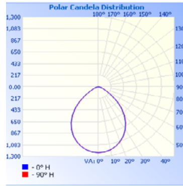
RT6S2500UNHD9SC3WH (5000K)
