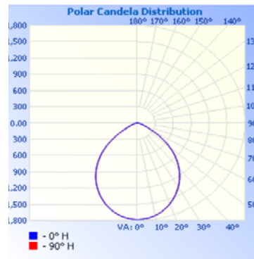
RT8S3500UNVD9SC3WH (2700K)
