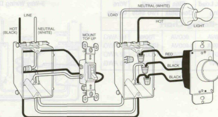
Rotary Dimmer 3-Way Wiring Diagram
