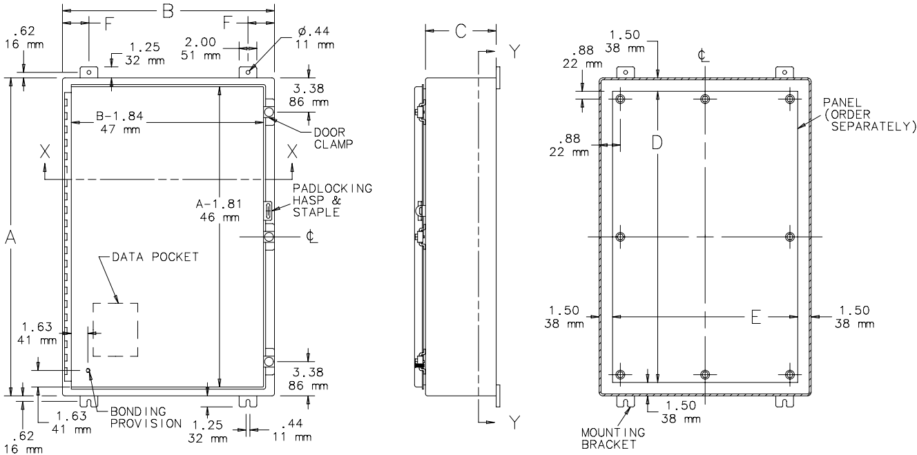
SECTION Y-Y
