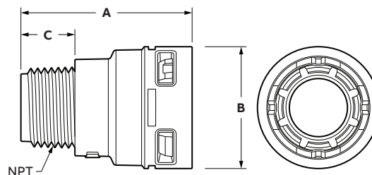
Threaded male terminal adapter
