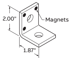
AB202M AB202M EG 90° bracket (2 hole)
