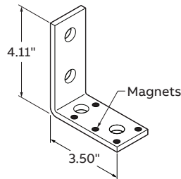
AB205M AB205M EG 90° bracket (4 hole)
