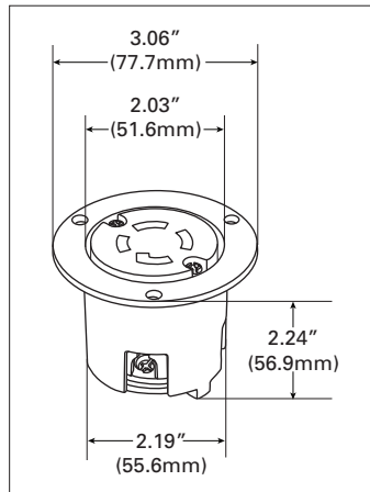
Figure 5. AHL1530FO
