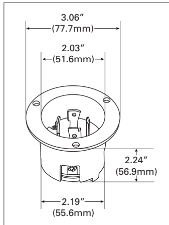
Figure 6. AHL1530FI
