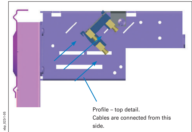
Detail 2 – profile
