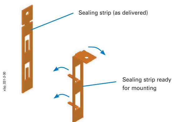
Detail
