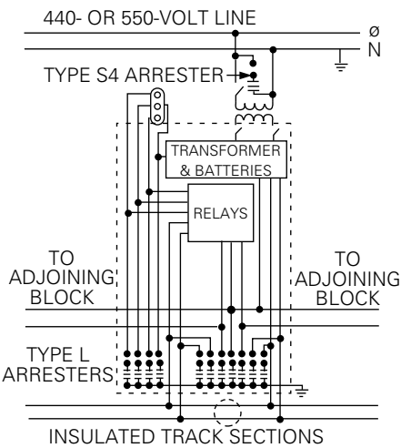
Figure 2. Railway application diagram showing an automatic railway block signal control with Type L secondary arresters. One arrester is used on each outgoing line.
