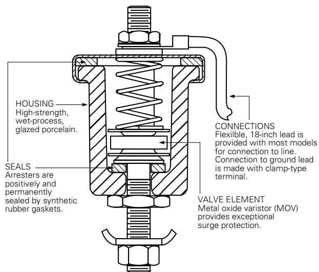
Figure 5. Cutaway illustration Type S4, 650 V secondary arrester.
