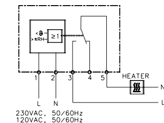
CONNECTION DIAGRAM
