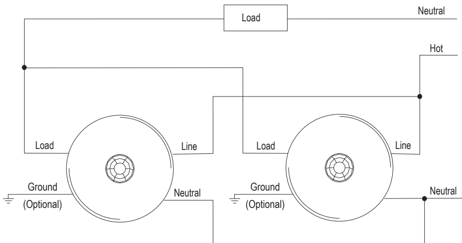
Multiple Sensors Connected in Parallel
