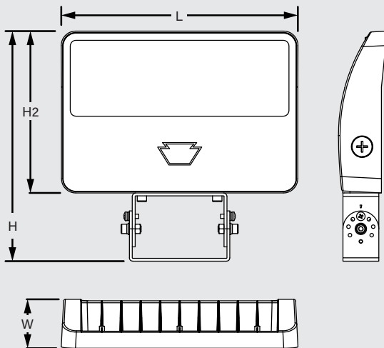
FIXTURE WITH TRUNNION MOUNT
