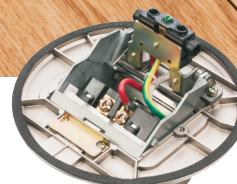
Brass Trapdoor style FLBT6615MB (open and back)
