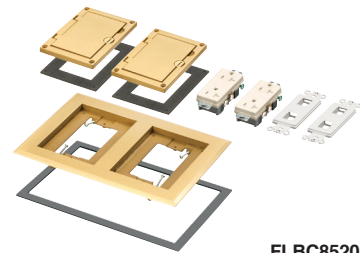
FLBC8520MB Two-gang Brass-plated
