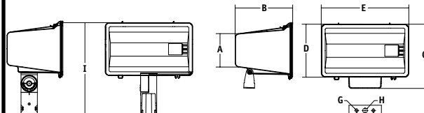
MHS KNUCKLE MOUNT
