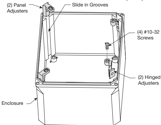
Hinged Adjuster
