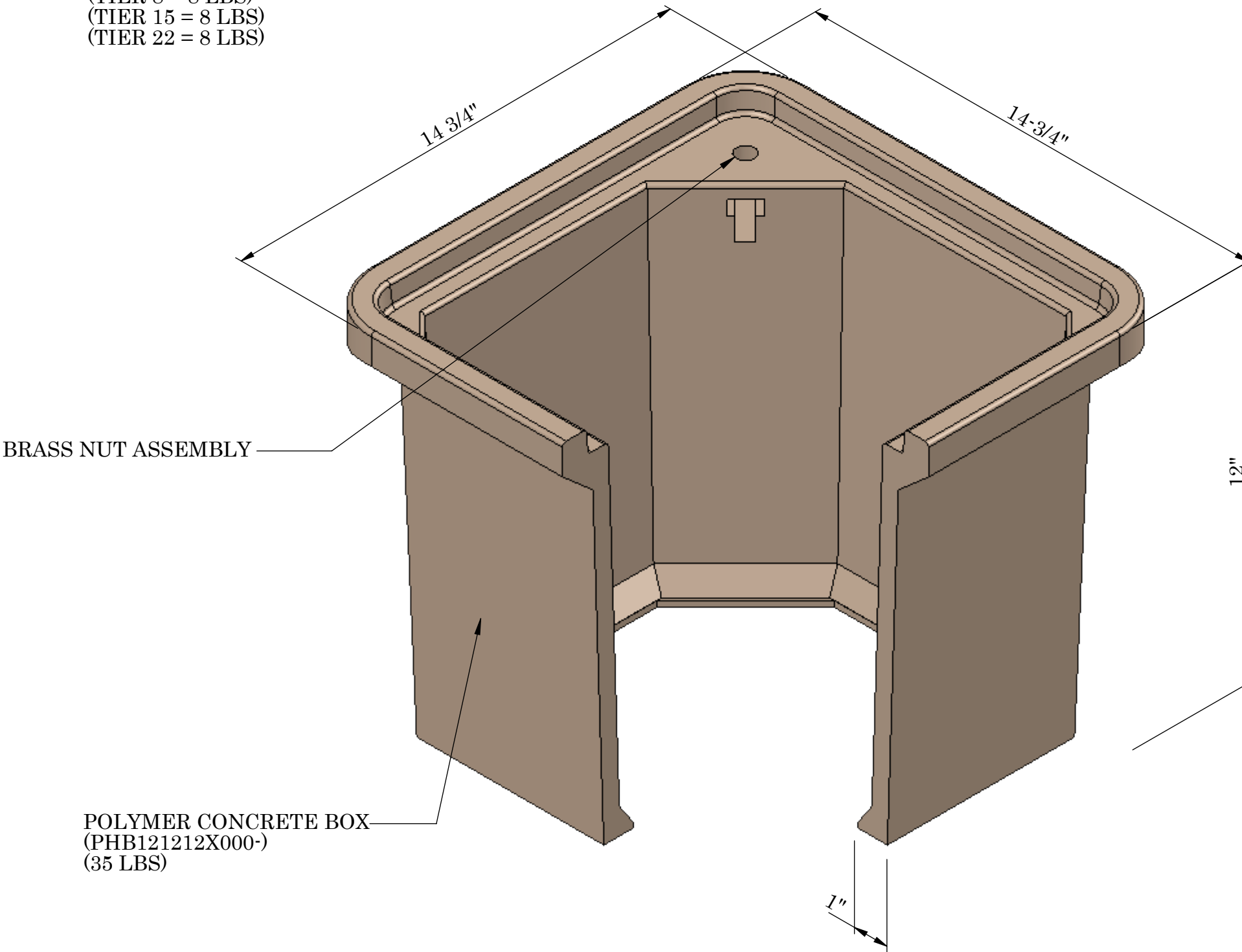
ISOMETRIC VIEW
