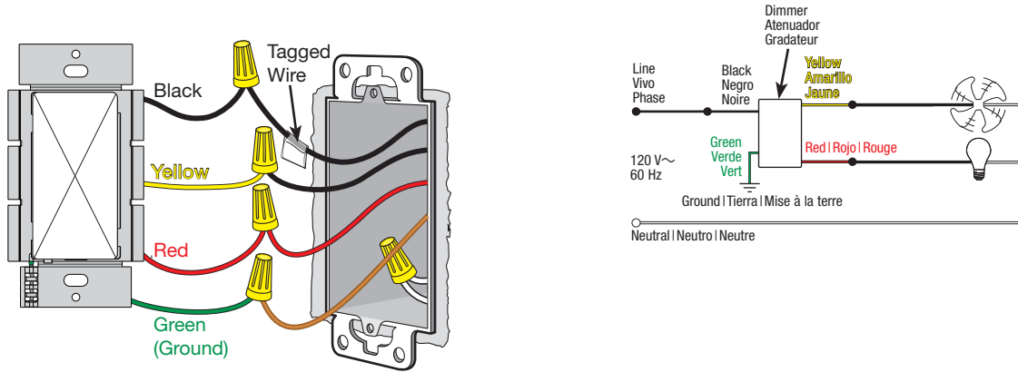
Image #30 — Dual Fan/Light Control with One Black Wire, One Red Wire and One Yellow Wire in a Single Pole Application
