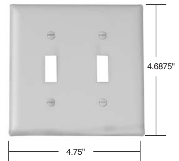
Dimensions for TradeMaster Two Gang
