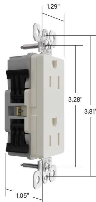
Depth (into Wallbox) = 1.05" TR26342DVSLA
