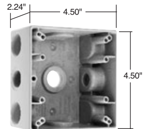
Dimensions for Two Gang Box
