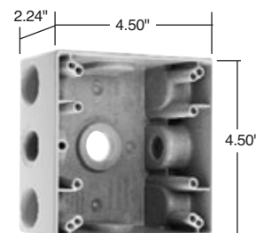
Dimensions for Two Gang Box
