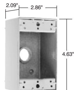
Dimensions for Single Gang Box
